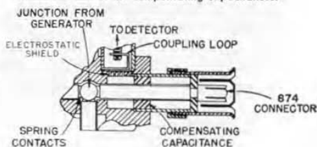
Figure 7. Sketch of modified junction showing the location of one of the compensating capacitances.
