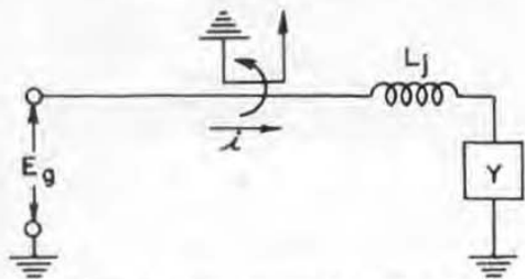
Figure 5c. Revised circuit of Figure 5b, with junction inductance shifted to the load side of the coupling loop.
