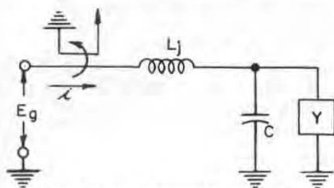
Figure 5d. Equivalent circuit showing the location of the compensating capacitance.
