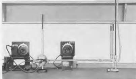
Figure 2. View of the Admittance Meter and balun as assembled for the measurement of a balanced transmission line.
