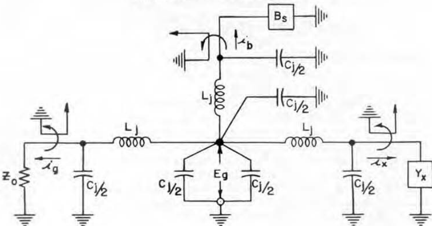
Figure 5a. Equivalent circuit of the junction.
